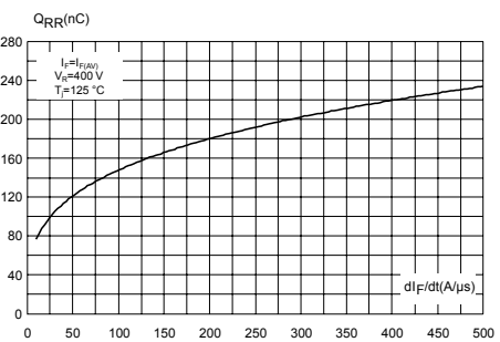
Figure 6. Reverse recovery charges versus di_F/dt (typical values)
