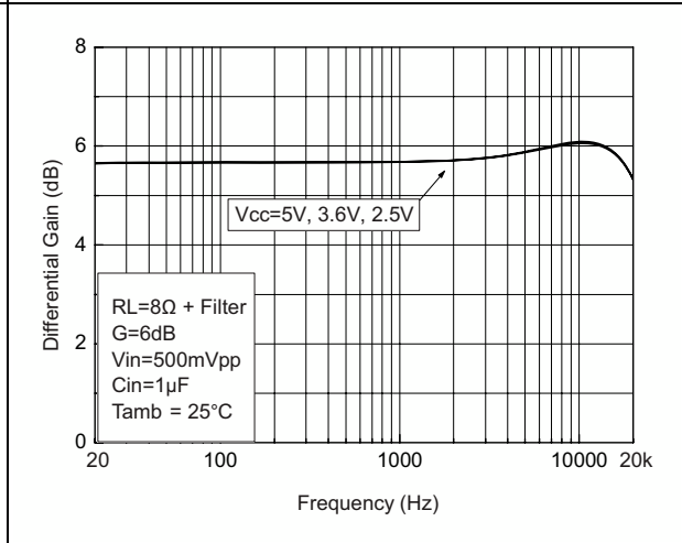
Figure 53. Gain vs. frequency
