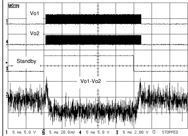
Figure 60. Startup and shutdown times V_{CC} = 3V , G = 6dB , No C_{in} (5ms/div)
