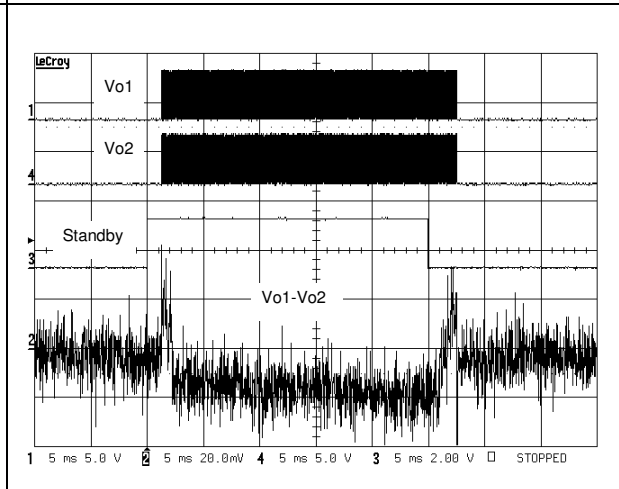
Figure 55. Startup and shutdown times V CC = 5V, G = 6dB, C in = 1μF (5ms/div)
