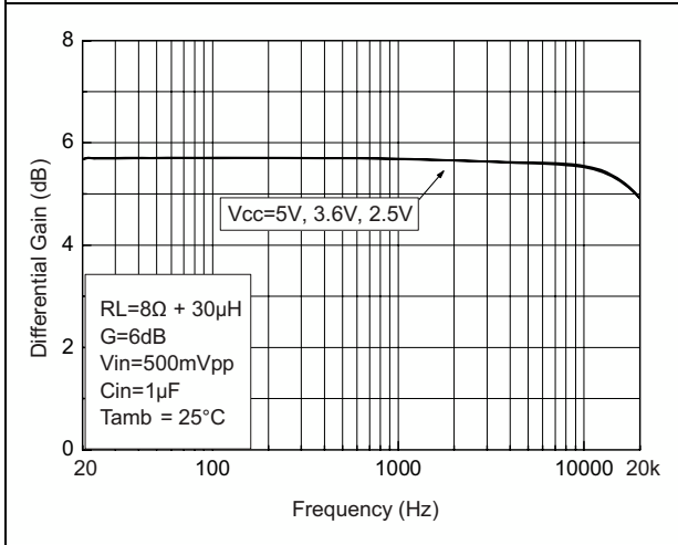
Figure 52. Gain vs. frequency
