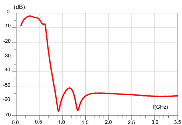
Figure 5. Transmission
