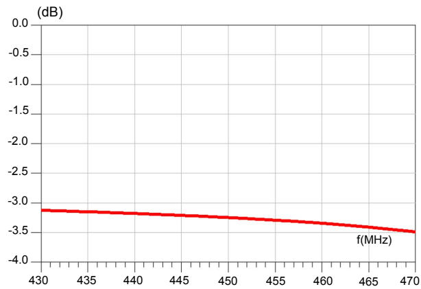
Figure 6. Insertion loss
