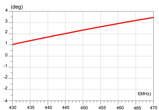
Figure 4. Phase imbalance
