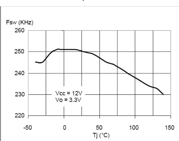
Figure 20. Switching frequency vs. junction temperature
