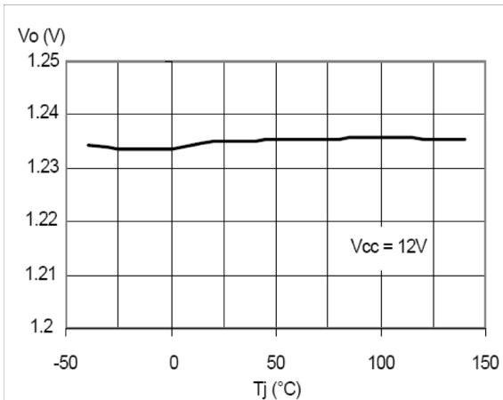
Figure 19. Output voltage vs. junction temperature
