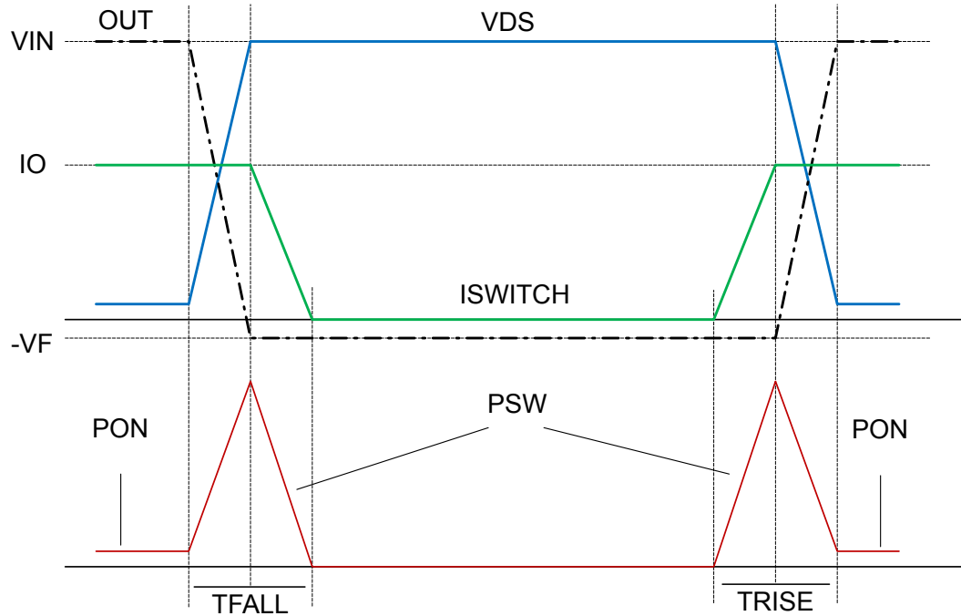
Figure 10. Switching losses
