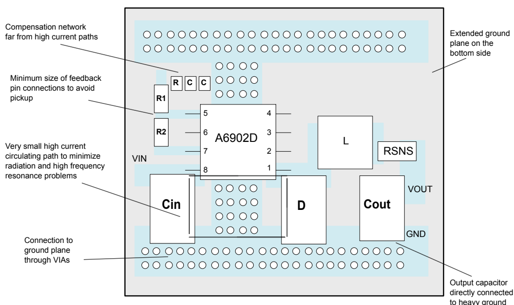
Figure 12. Layout example
