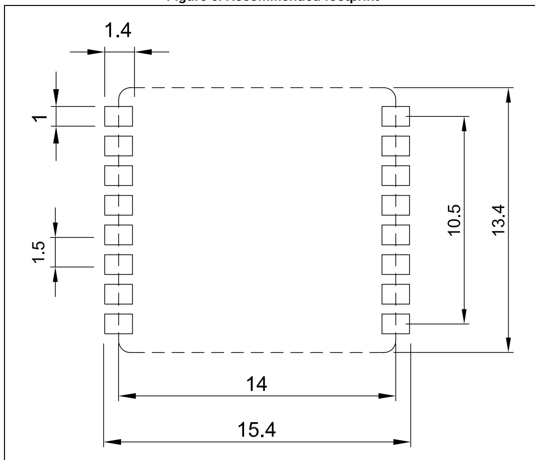
Figure 6. Recommended footprint
