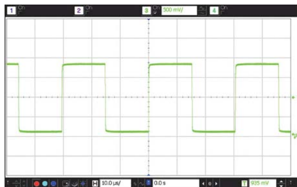
Figure 4. LVCMOS Waveform (V dd = 1.8V) into 15 pF Load
