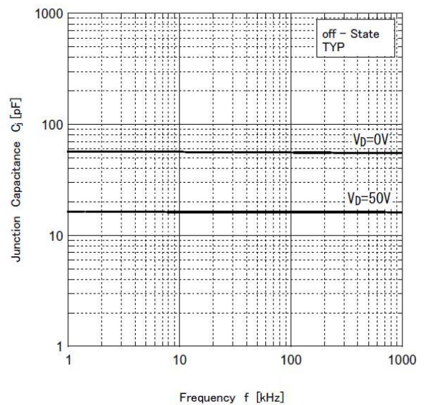
Junction Capacitance
