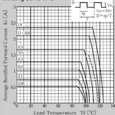
Derating Curve T_J - I_o
