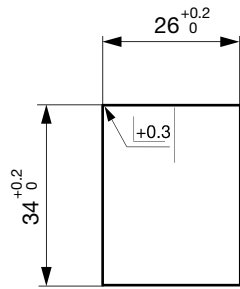
Panel cut-out 2 Pole
