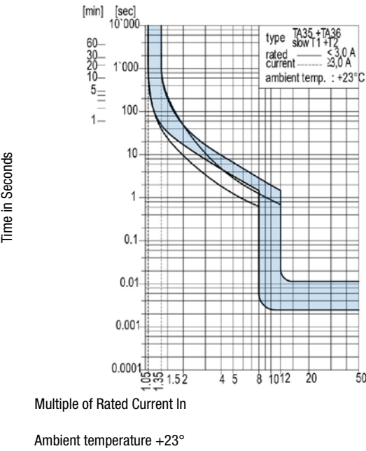
Tripping Characteristics thermal magnetic time lag
