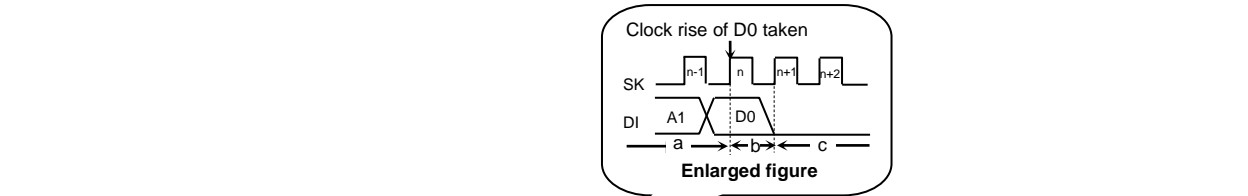
Figure 41. READ cancel available timing
