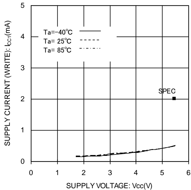
Figure 14. Supply Current (WRITE) vs Supply Voltage ( f_{sk}=3\text{MHz} )
