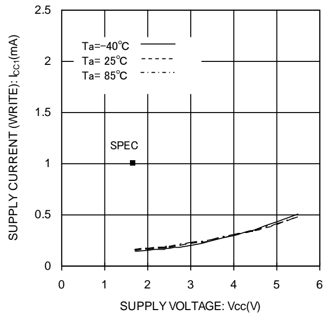
Figure 13. Supply Current (WRITE) vs Supply Voltage ( f_{sk}=1\text{MHz} )
