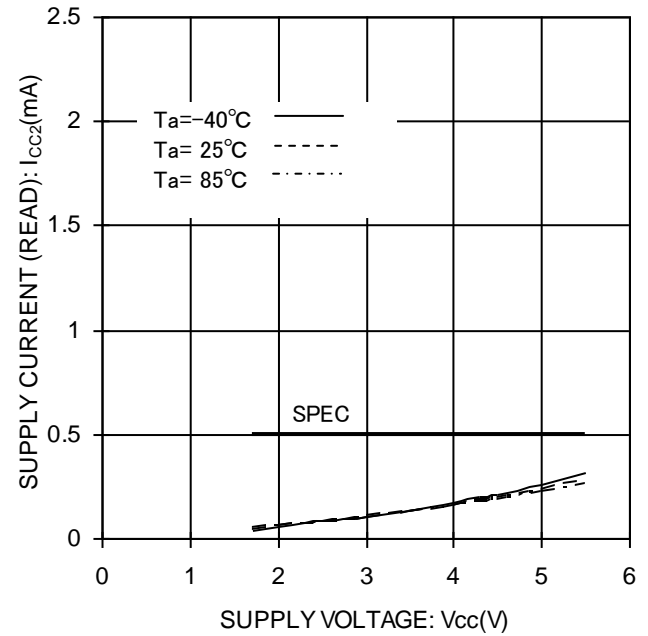
Figure 15. Supply Current (READ) vs Supply Voltage ( f_{sk}=1\text{MHz} )
