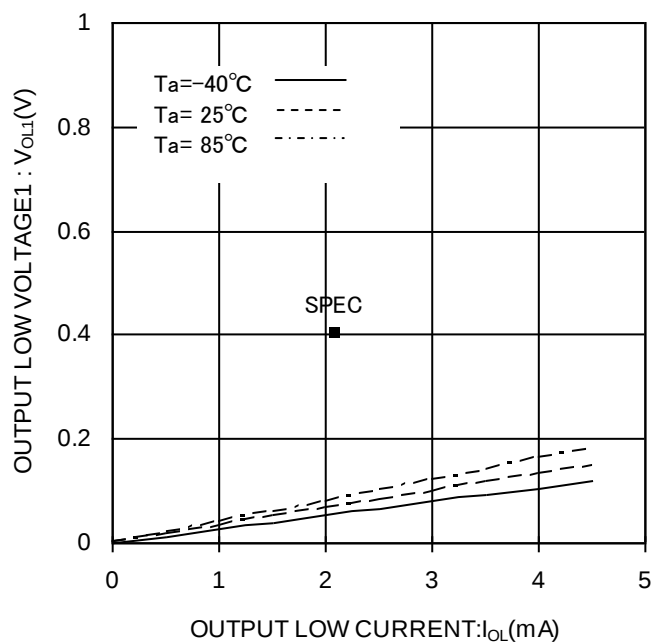
Figure 6. Output low voltage1 V_{O1} (VCC=2.7V)
