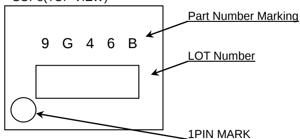
SOP8(TOP VIEW)
