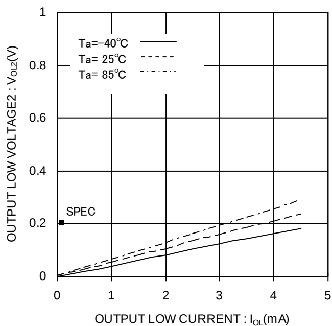
Figure 7. Output low voltage2 V_{O2} (VCC=1.7V)
