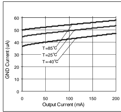
Fig.51 IOU - IGND
