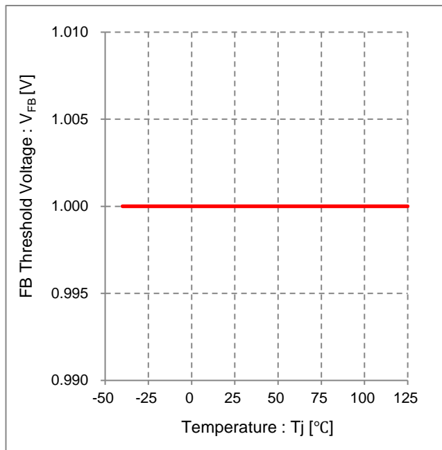
Figure 3. FB Threshold Voltage vs Temperature
