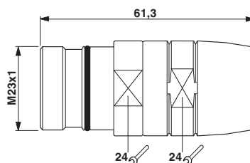
Dimensional drawing
