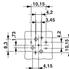
Drilling diagram
