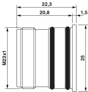
Dimensional drawing
