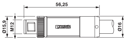
Plug, M12 x 1, straight, shielded
