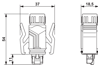
Dimensional drawing
