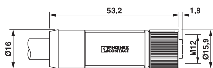
M12 x 1 socket, straight
