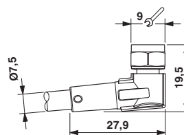
Dimensional drawing
