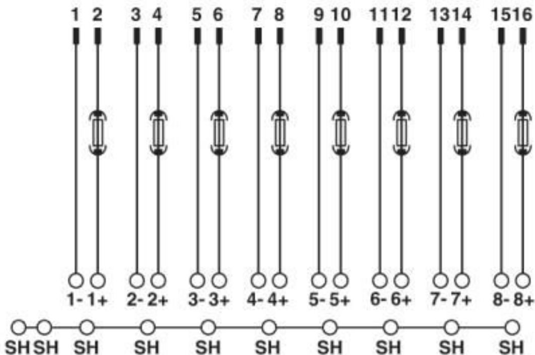
Connection scheme UM-DELTA V/D/SI/BFI/TP
