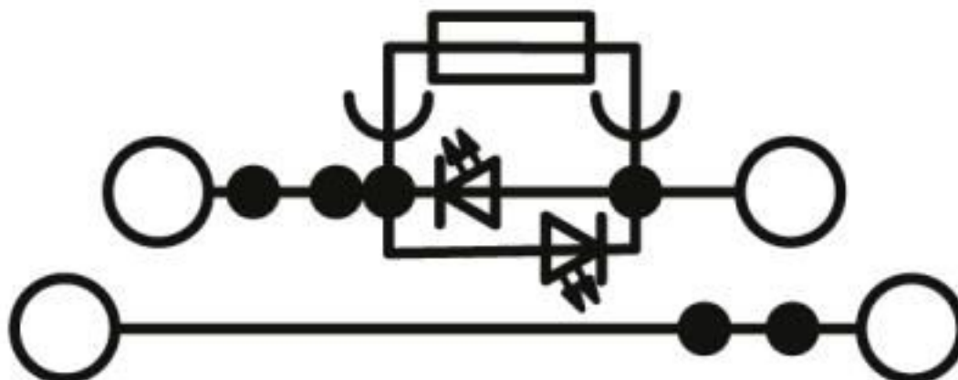
Circuit diagram
