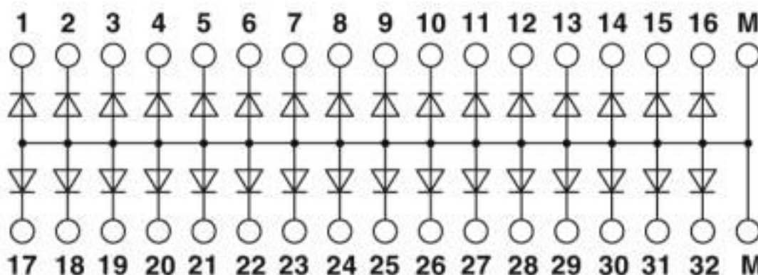
Circuit diagram
