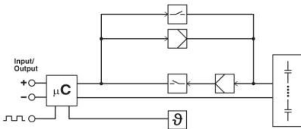
Block diagram
