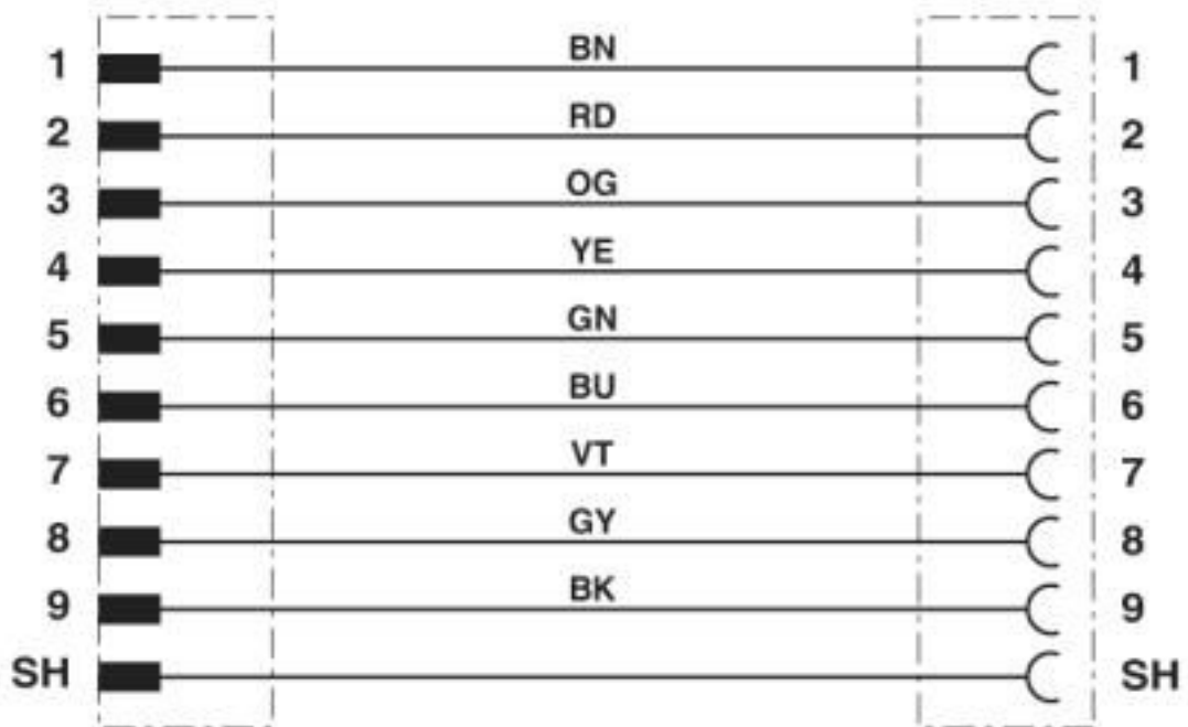
Circuit diagram
