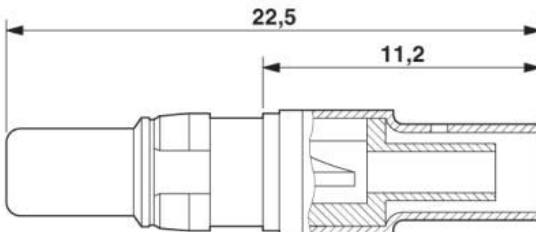
Dimensional drawing
