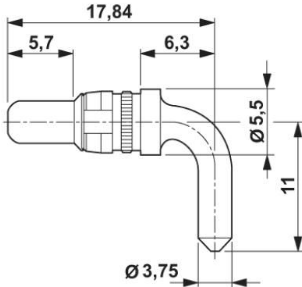
Dimensional drawing
