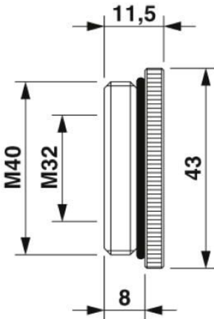
Dimensional drawing
