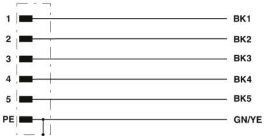
Circuit diagram
