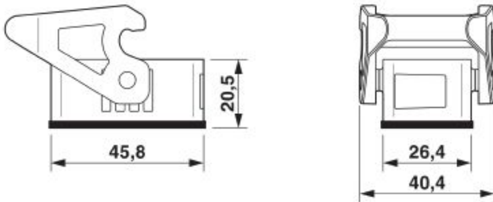
Dimensional drawing
