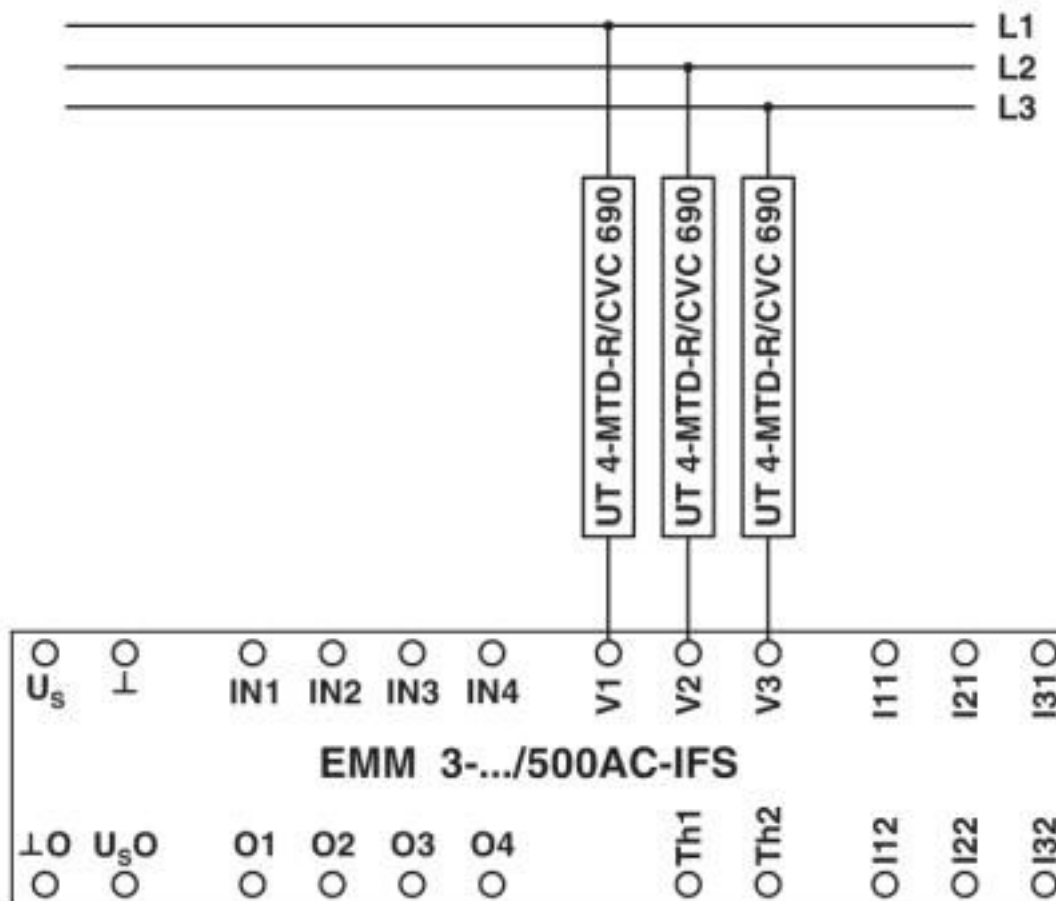
Connection diagram
