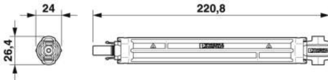
Dimensional drawing
