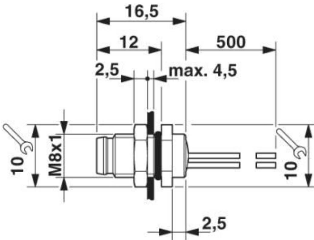
Dimensional drawing
