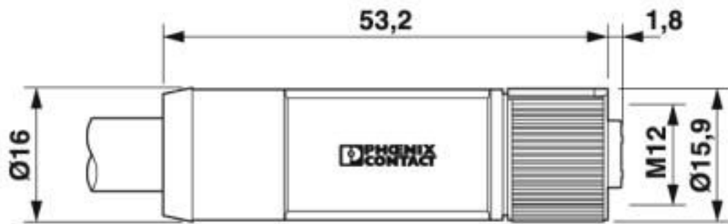
M12 x 1 socket, straight
