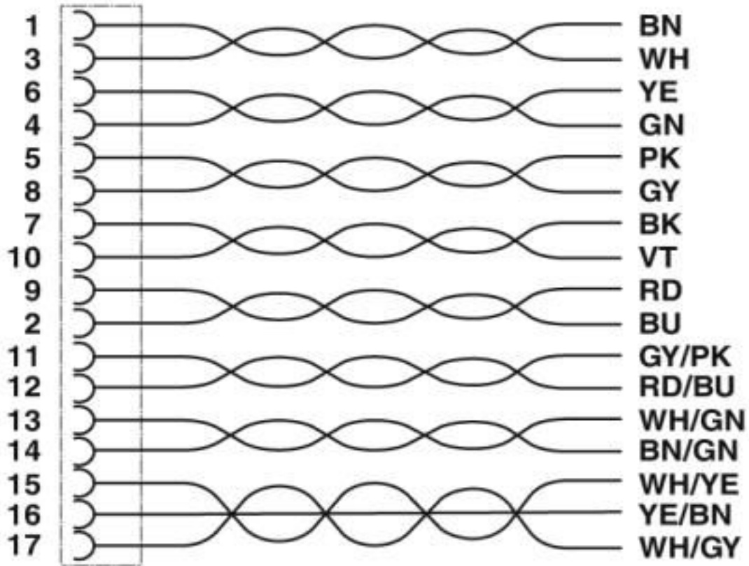
Circuit diagram
