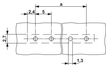
Drilling diagram
