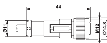
Dimensional drawing
