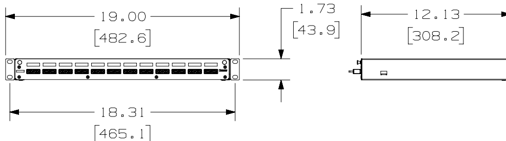
12 PORT SHOWN
