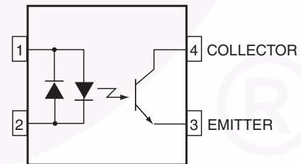
Equivalent Circuit
