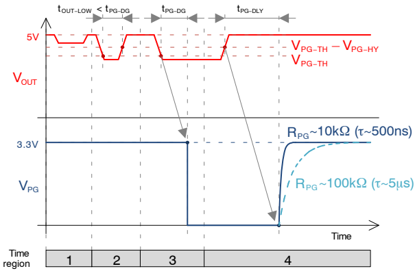
Figure 80. Timing – PG Connected to Application Power Supply 3.3 V
