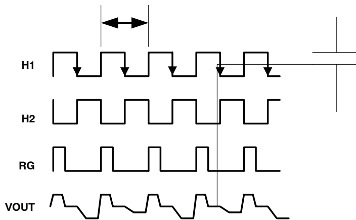
Figure 21. Pixel Timing
