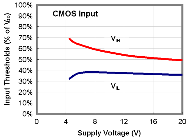
Figure 23. Input Threshold % vs. Supply Voltage
