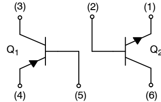
SOT-363 CASE 419B STYLE 1
