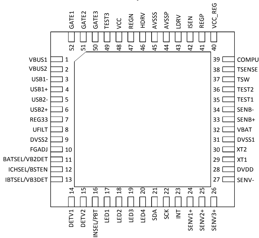
Figure 4: Pin Assignment
