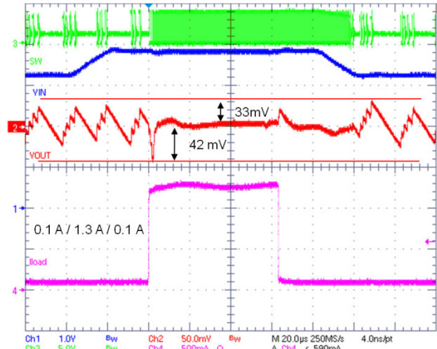
Figure 28. Transient Load 0.2 to 1.5 A – Single Shot Transient Line 3.3 to 3.9 V – Auto Mode
