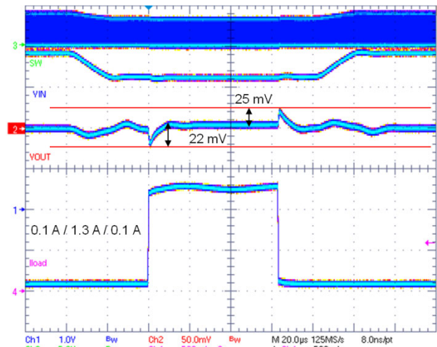
Figure 30. Transient Load 0.1 to 1.4 A – Multi Shot Transient Line 3.9 to 3.3 V – PWM Mode
