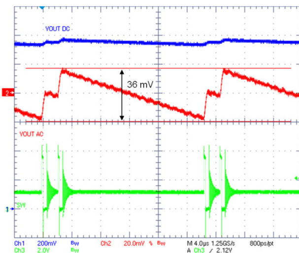
Figure 25. PFM Ripple
