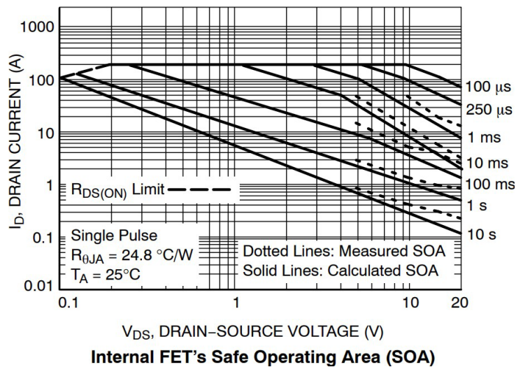
Figure 35. Power FET Safe Operating Curves
