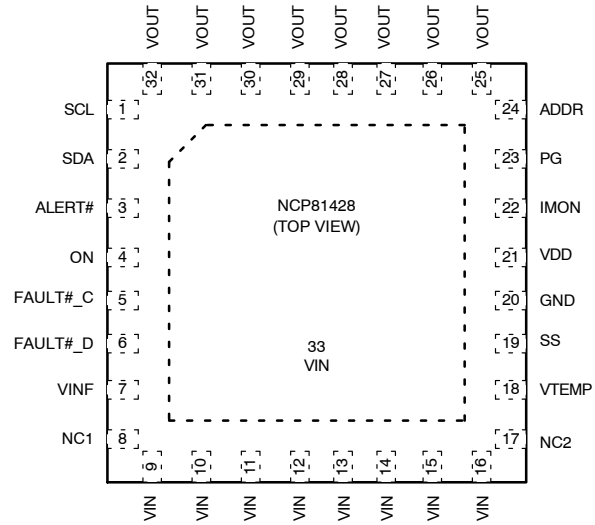
Figure 6. Pin Connections
