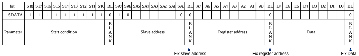
Figure 7 : 2-wire Serial Communication Frame
