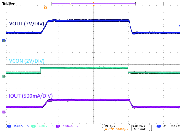
Figure 15. V_{CON} Transient (PFM to PWM), V_{OUT} = 1.4\text{ V} to 3.4\text{ V} , R_{LOAD} = 6.8\ \Omega , V_{IN} = 3.8\text{ V} , 100 ns Edge
