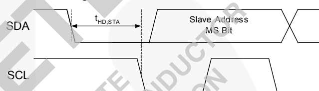
Figure 40. Start Bit
