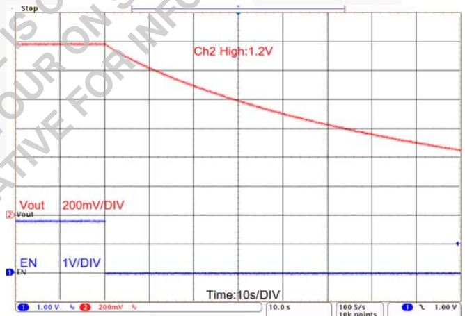
Figure 30. Shutdown, Output Discharge Off
