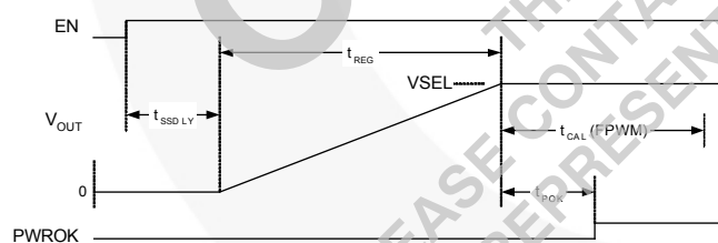
Figure 35. Soft-Start Timing
