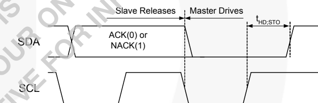
Figure 41. Stop Bit
